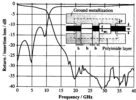
Fig. 2. Set-up and results of low-pass filter ( w = 0.2 mm, w + 2s = 0.456 mm, w_1 = 0.02 mm, l_1 = 0.118 mm, l_2 = 1.246 mm, l_3 = 0.174 mm).
