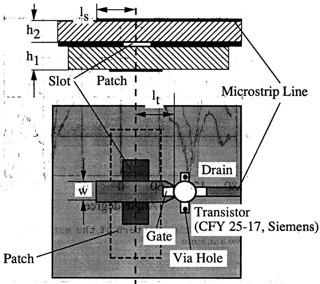
Fig. 1: Basic configuration of the active antenna (Patch 8x12 mm, slot 0.5x4.6 mm, \epsilon_{r1}=2.33 , \epsilon_{r2}=10.8 h_1=1.57\text{mm} , h_2=0.64\text{mm} , l_s=1.1\text{mm} , w=2.577\text{mm} ( 20\Omega ), l_t=2.0\text{mm} ).
