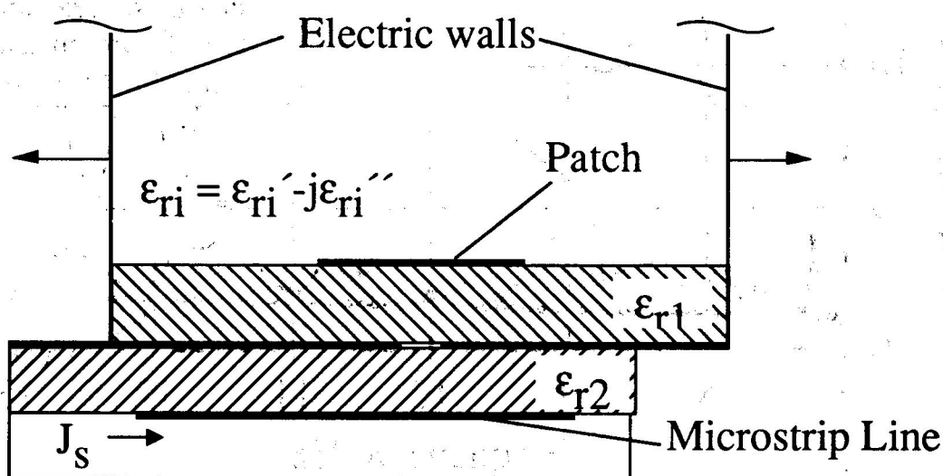
Fig. 2: Equivalent structure for theoretical analysis of the passive antenna
