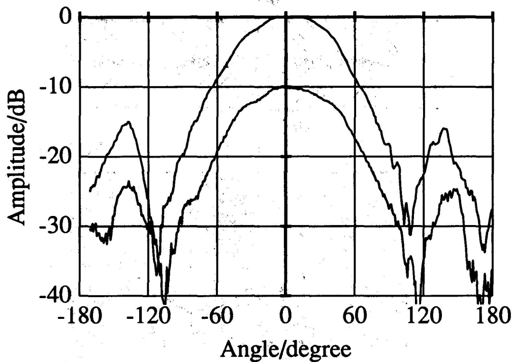
Fig. 3: H-plane radiation pattern of the active and passive antenna
