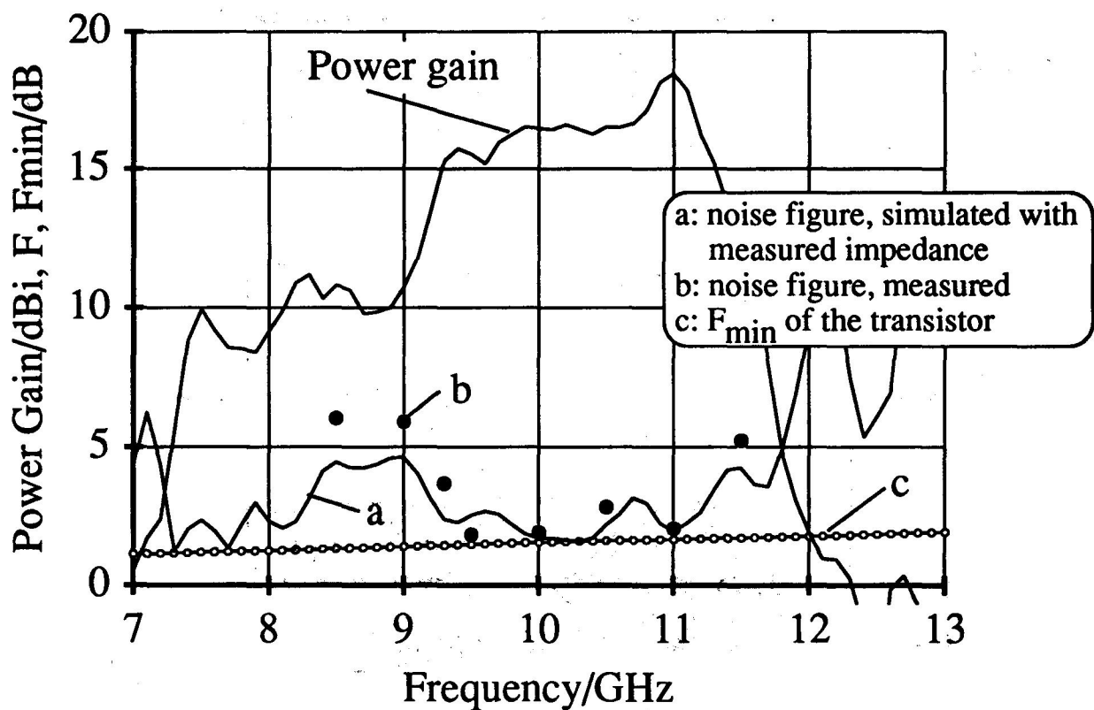
Fig. 4: Power gain and noise figure of the active antenna
