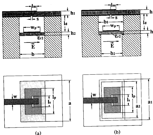
Fig. 1. Basic (a) and modified (b) configuration of new waveguide to microstrip transition.
