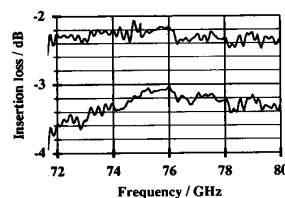
Fig. 5. Comparison of two sets of transitions with different microstrip line lengths ( l_1 = 21.4 mm, l_2 = 31.4 mm).
