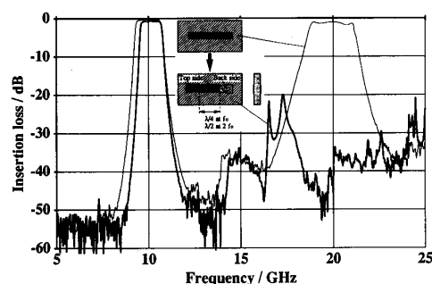
Fig. 3. Wide-band performance of 10 GHz suspended stripline bandpass filter. Thin line: standard design as in Fig. 2; fat line: resonators replaced by double strip structure.
