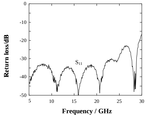
Fig. 6: Return loss of a homogeneous microstrip line after deembedding the via-less prober contact (Dimension according to Fig. 5).
