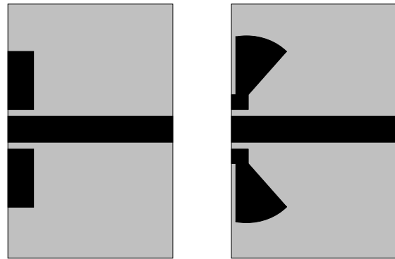
Fig. 3: Rectangular and radial stubs to provide the RF ground connection.
