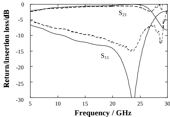
Fig. 5: Theoretical (—) and experimental (---) results for a transition using radial stubs
