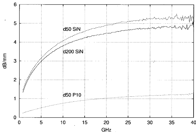
Fig. 11. Loss of coplanar lines on top of a dielectric on standard silicon ( 5\text{--}20\ \Omega\text{cm} ). d50 SiN and d200 SiN denote a 200-nm \text{Si}_3\text{N}_4 dielectric and 50- \mu\text{m} or 200- \mu\text{m} ground spacing, respectively. d50 P10 denotes a 10- \mu\text{m} polyimide dielectric and 50- \mu\text{m} ground spacing.
