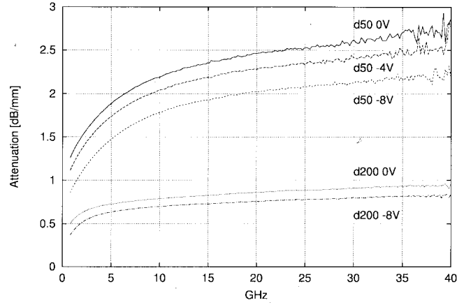
Fig. 8. Losses of coplanar lines on top of silicon ( 2000 \Omega\text{cm} ) with a 200\text{-nm} Si 3 N 4 passivation layer, also with bias voltage applied between center conductor and ground plane ( -4\text{ V} , -8\text{ V} ).
