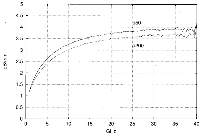
Fig. 10. Loss of coplanar lines on standard silicon 5\text{--}20\ \Omega \cdot \text{cm} .
