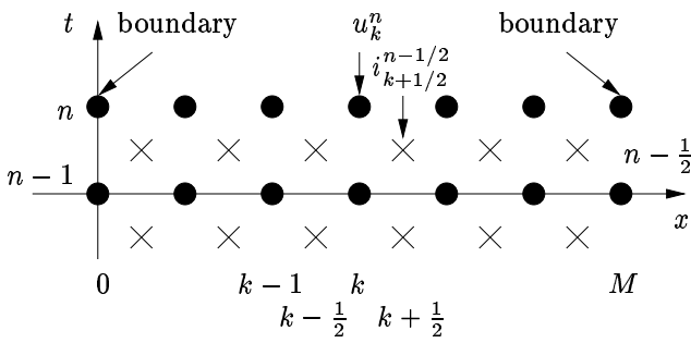
Fig. 2. Numerical domain of the leapfrog scheme
