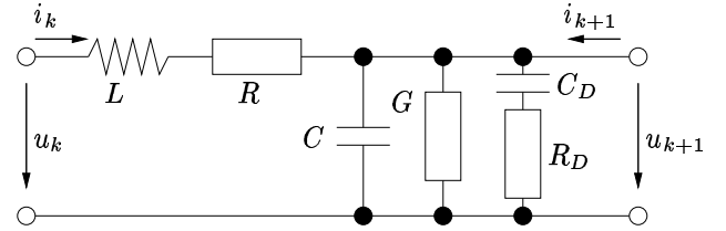
Fig. 8. Model of a nonlinear transmission line
