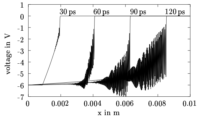
Fig. 9. Shock formation on the GaAs NLTL excited with a step function with 20 ps fall time; signal on the NLTL after 30 ps, 60 ps, 90 ps and 120 ps using the leapfrog scheme.
