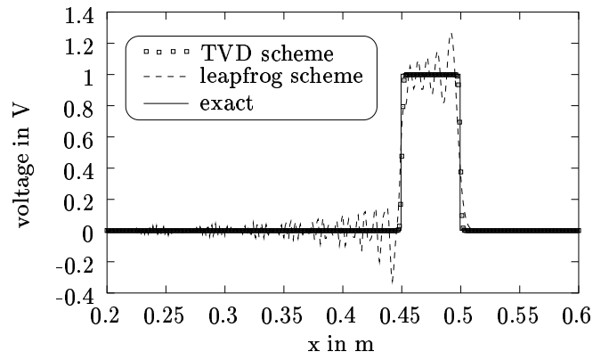
Fig. 4. Propagation of a rectangular pulse (0.167 ps) on a linear transmission line ( 50 \, \Omega , \beta = c_0 ); comparison between the leapfrog and TVD scheme after 1000 time steps; CFL-number=0.5.
