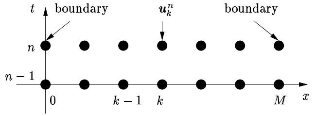
Fig. 1. Numerical domain of the TVD scheme
