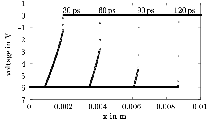
Fig. 10. Shock formation on the GaAs NLTL excited with a step function with 20 ps fall time; signal on the NLTL after 30 ps, 60 ps, 90 ps and 120 ps using the TVD scheme.
