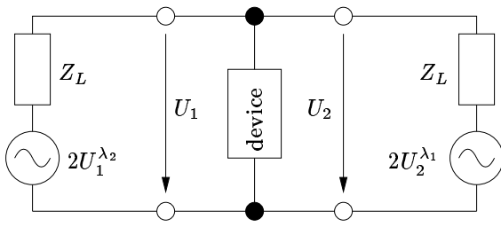
Fig. 5. Equivalent circuit for the computation of the scattering problem of the lumped element in the time domain.
