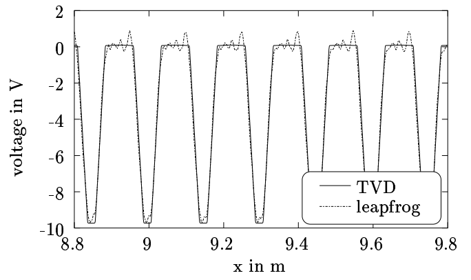
Fig. 7. Propagation of a scattered harmonic signal (2 GHz) on a 10 m long transmission line ( 50 \Omega , \beta = c_0 ) loaded with a diode placed in the middle of the line after 20000 time steps (Courant-number=0.5).
