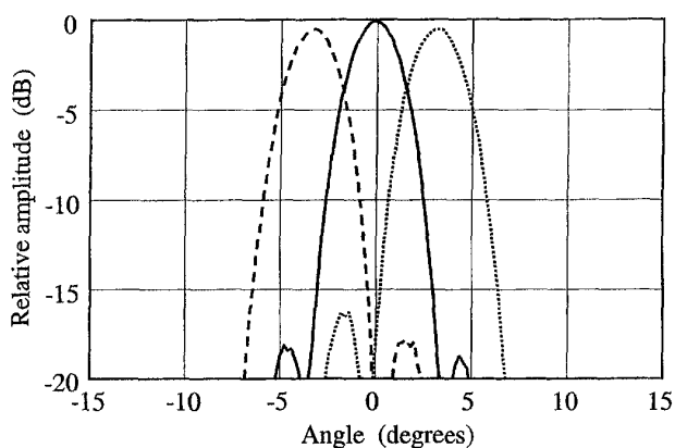
Figure 12b. Details of the scanning performance for the antenna of Figure 12a.
