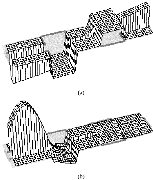
Fig. 11. Electric-field distribution in a three-element low-pass filter. (a) Low-frequency (passband). (b) Frequency of maximum attenuation (input from the left-hand side).
