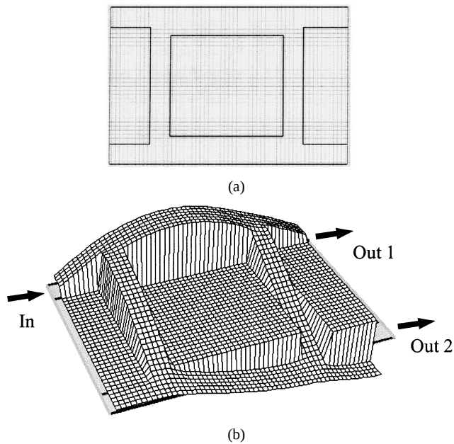
Fig. 9. Basic layout and field distribution in a microstrip hybrid-ring coupler.
