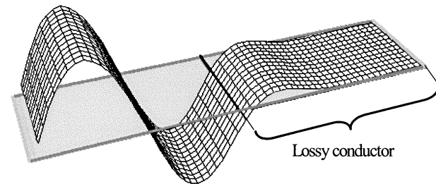
Fig. 3. Plane wave incident on a lossy conductor.
