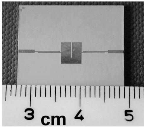
Fig. 8. Photograph of the folded microstrip filter (coupling length: 4.63 mm, length of first resonator: 5.25 mm, length of second resonator: 4.88 mm, height of central resonator: 4.5 mm, lateral dimension of central resonator: 4.25 mm, slot in central resonator: 3.25 mm \times 0.25 mm, all other data as in Fig. 3).
