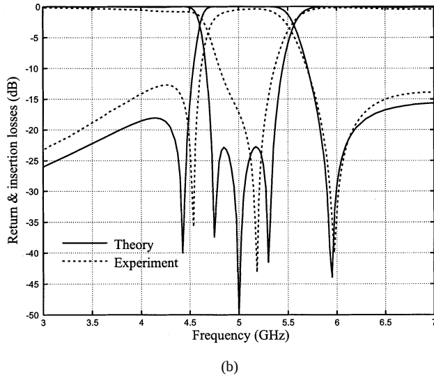
Fig. 4. Theoretical and experimental results of an optimally designed stub-tapped microstrip filter sample. (a) Dimensional layout. (b) Return and insertion losses.
