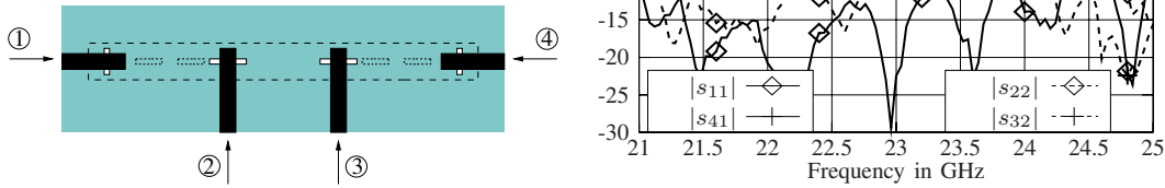
Fig. 3. Measurement of the dual mode transition from NRD-guide to microstrip line: left setup, right S-parameters.
