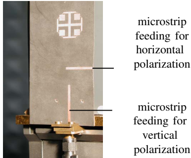
Fig. 7. Photo of the dual polarization antenna.
