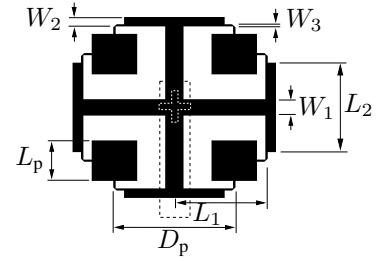
Fig. 6. Setup of the dual polarization radiating element.
