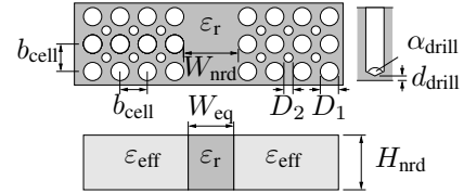
Fig. 1. SINRD-guide topology: at the top drilling hole pattern, at the bottom equivalent NRD-guide for faster simulations.
