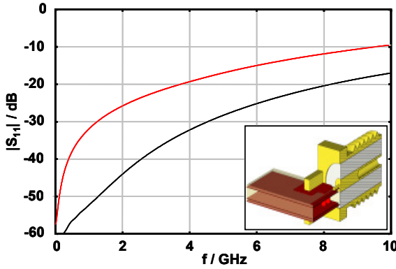
Fig. 4: Simulation results for old (red) and new (black) transitions from SMA connector to MSL; perspective drawing of the transition.
