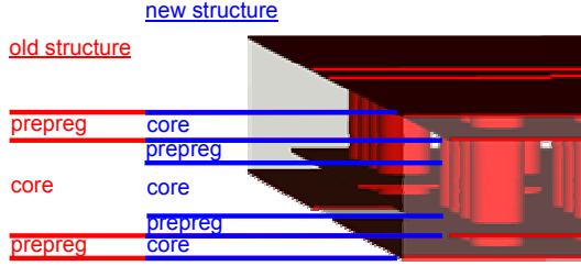
Fig. 3: Old and new layer stack of test PCBs.
