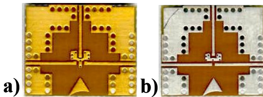
Fig. 5: Top view of test PCBs providing a neutral environment to SAW filters with unbalanced input and balanced output, (a) in 1.6 mm x 2.0 mm 6-pin, and (b) in 1.4 mm x 2.0 mm 5-pin packages.
