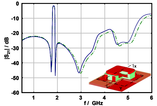
Fig. 6: Comparison of simulated scattering parameters of identical filters on optimized test PCB (green, dash-dotted) and new quasi-application PCB (blue, solid).
