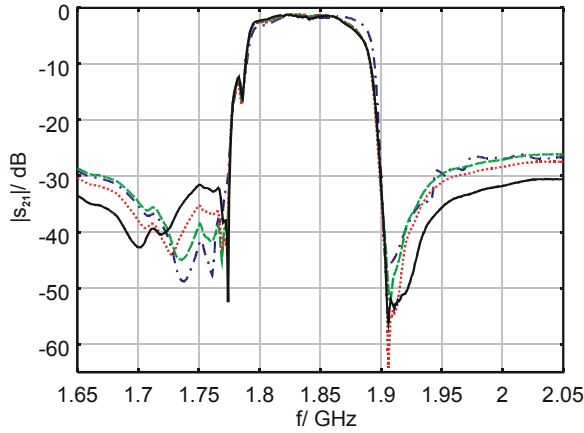
Fig. 1: Measured scattering parameters of identical filters on three different PCBs ((1) green-dashed, (2) red-dotted, (3) black-solid) and simulated values (blue-dash-dotted) of the same filter on the PCB used for measurement (1).
