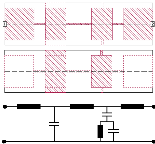
Fig. 9: Layout and equivalent circuit of a low-pass filter with modified capacitance element.
