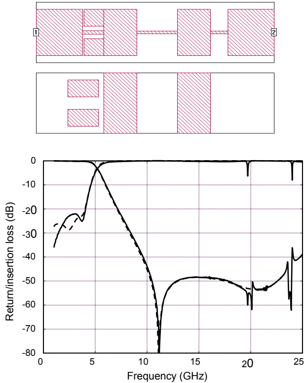
Fig. 6: Front and backside layout and transmission performance of a low-pass filter with a single edge capacitive coupling. (Dashed lines: theory, solid lines: experiment).
