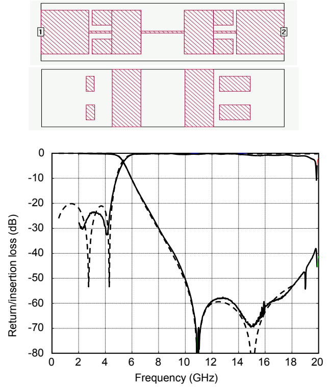
Fig. 7: Front and backside layout and transmission performance of a low-pass filter with a twofold edge capacitive coupling. (Dashed lines: theory, solid lines: experiment).
