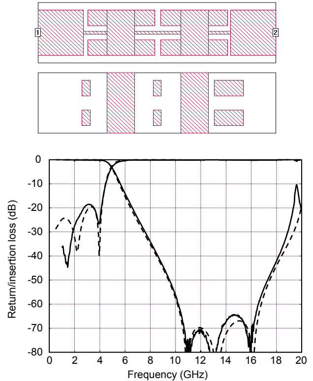
Fig. 8: Front and backside layout and transmission performance of a low-pass filter with a threefold capacitive coupling. (Dashed lines: theory, solid lines: experiment)
