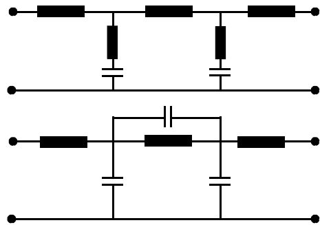
Fig. 2: Equivalent circuits of possible quasi-elliptic low-pass filters.
