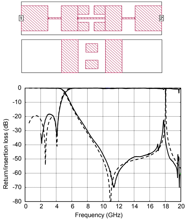
Fig. 5: Front and backside layout and transmission performance of a low-pass filter with a single central capacitive coupling. (Dashed lines: theory, solid lines: experiment).
