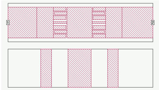
Fig. 3: Front side (top) and back side (bottom) layout of a quasi-elliptic low-pass filter using interdigital coupling.
