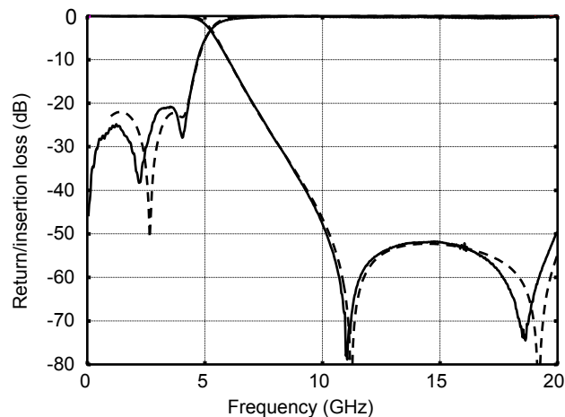
Fig. 10: Transmission performance of a low-pass filter with modified capacitance element. (Dashed lines: theory, solid lines: experiment).
