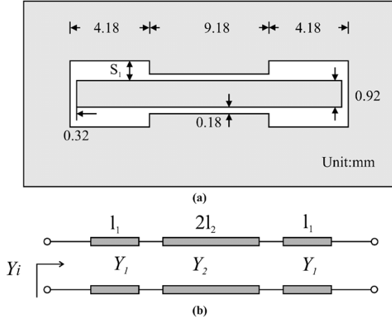
Fig. 2. Proposed MMR on coplanar waveguide. (a) Layout. (b) Equivalent transmission line network.
