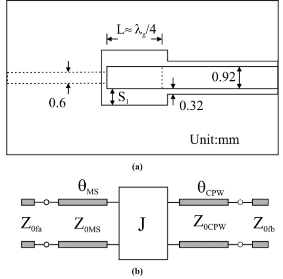
Fig. 3. Surface-to-surface microstrip/CPW coupling structure. (a) Layout. (b) Equivalent J-inverter network.
