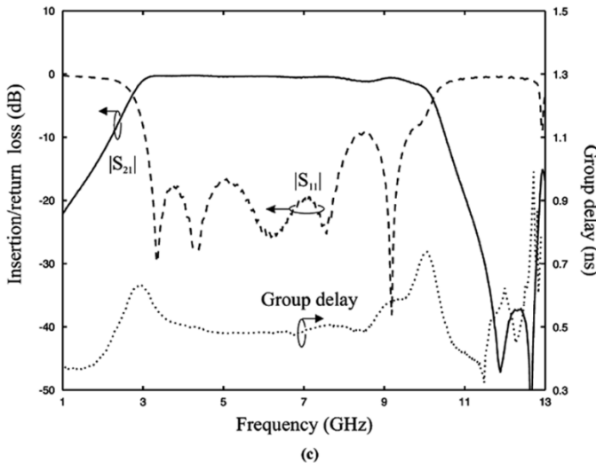
Fig. 6. Photographs and measured results of a fabricated UWB filter. (a) Top view. (b) Bottom view. (c) Measured S -magnitudes and group delay.
