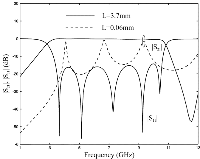
Fig. 5. Frequency responses of the proposed UWB BPF with the fixed slot width of S_1 = 1.1 mm and different lengths of L = 0.06 and 3.7 mm in the microstrip/CPW coupling sections.
