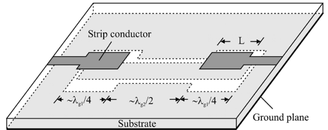
Fig. 1. Three-dimensional view of the proposed UWB BPF based on hybrid microstrip/CPW structure.
