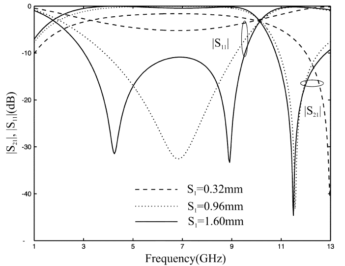
Fig. 4. Simulated S -parameters of the coupling structure in Fig. 3.
