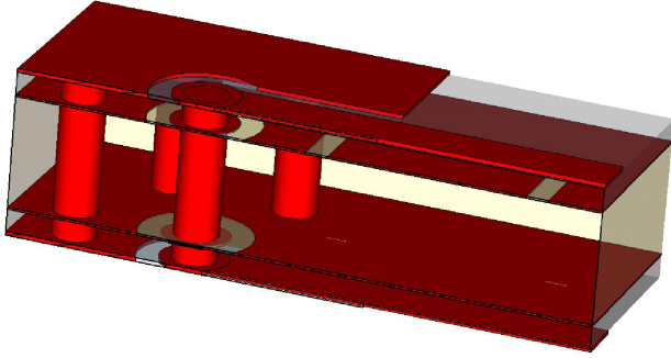
Fig. 4. Cross section view of the simulation model of the PCB feed-through.
