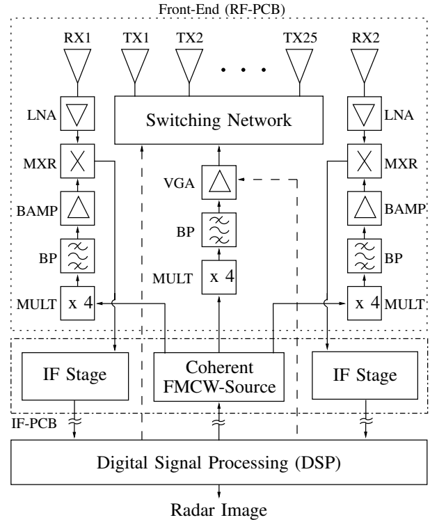
Fig. 1. Block diagram of the sensor front-end.
