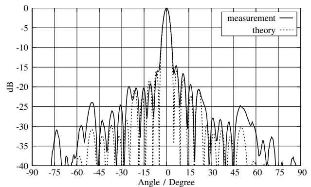
Fig. 7. Synthesized radiation diagram of the antenna array in azimuth at 24.5 GHz compared with theory.
