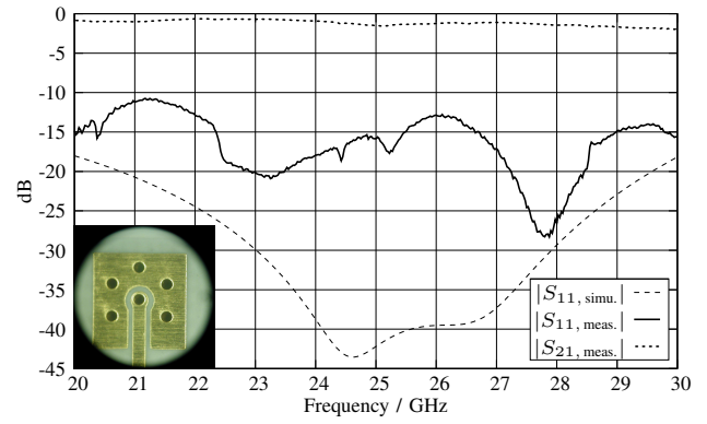
Fig. 5. Measured and simulated scattering parameters of the PCB feed-through (see microscope photograph).
