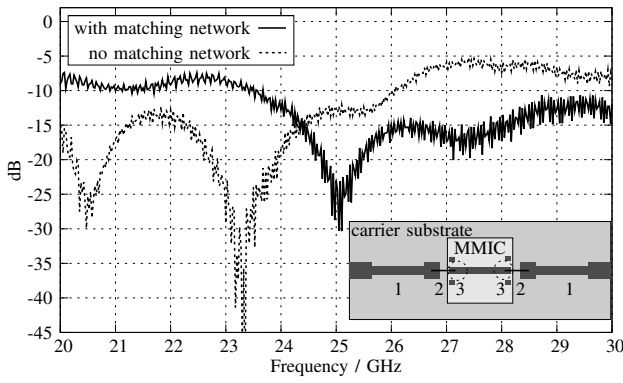
Fig. 3. Measured return loss of the MMIC connection with and without matching network. The inset in the diagram shows the top view of the case with the matching network (1: matching network, 2: bond wire, 3: carrier substrate ground via).
