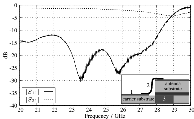
Fig. 6. Measured scattering parameters of the transition (see 2D cross section) between carrier substrate and antenna substrate (1: microstrip \lambda/4 -transformer, 2: soldered wire, 3: ground via).
