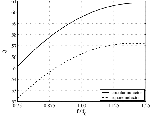
Fig. 7. Simulated quality factor of planar inductors.
