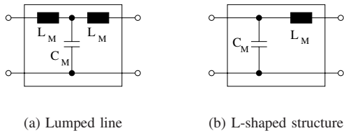
Fig. 3. Proposed lumped matching networks.
