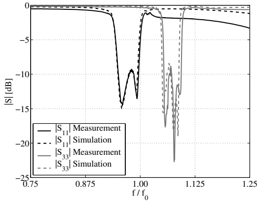
Fig. 9. Reflection properties of the SAW duplexer.
