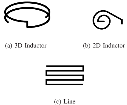
Fig. 6. Layout of matching elements (not drawn to scale).
