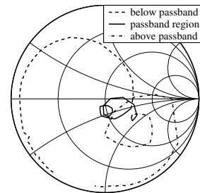
Fig. 2. Input reflection coefficient of a SAW filter.
