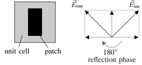
Fig. 3. 90^\circ -twist of polarization using cells with 180^\circ difference in reflection phases of orthogonal field components.
