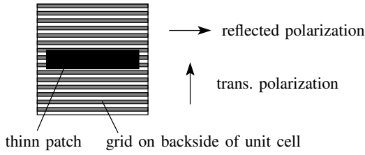
Fig. 2. Cell of the upper reflector with a thin dipole and a grid on the substrate backside, which acts as a ground plane for horizontal polarization and which is transparent for orthogonal polarization.
