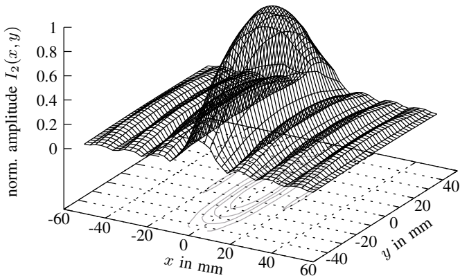
Fig. 5. Normalized amplitude distribution I_2 on the lower reflector with |si| -distribution along the x -axis and cosine-taper along the y -axis.
