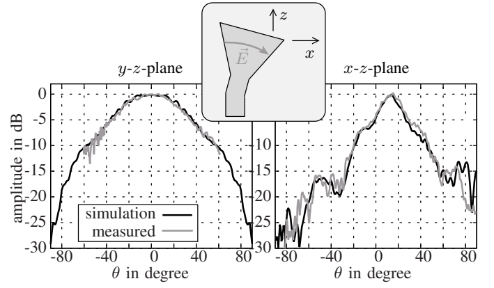
Fig. 6. far field characteristic of the rectangular feed horn in the H- and E-plane at 58 GHz.
