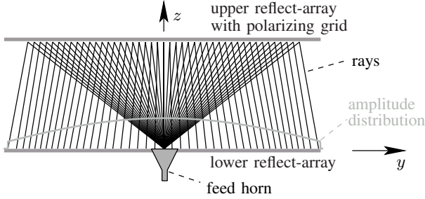
Fig. 9. (Projected) Rays in the y - z -plane.
