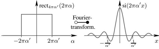
Fig. 4. Idealized sector-characteristic with sector-angle \Delta\theta ( \alpha' = \sin(\Delta\theta/2)/\lambda , \alpha = \sin \theta/\lambda ) and si-shaped amplitude distribution which is its Fourier-transform.
