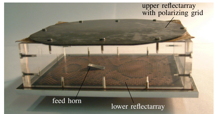
Fig. 11. Photograph of the fabricated double-reflectarray.
