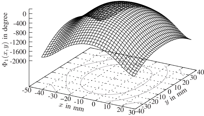
Fig. 10. Calculated reflection phase \Phi_1(x_1, y_1) on the upper reflector.
