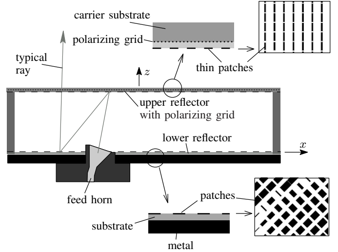
Fig. 1. Cross section of a dual-reflectarray-setup.
