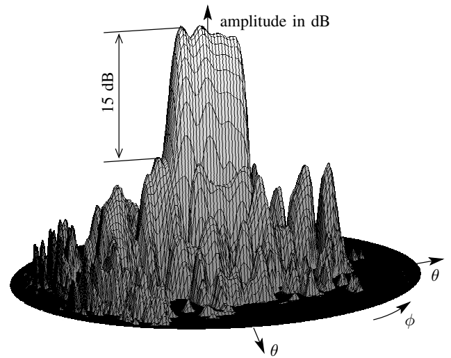
Fig. 14. Measured normalized far field characteristic at 57.6 GHz from -35 dB to 0 dB.
