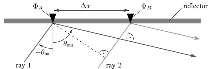
Fig. 7. Reflection of rays at a one-dimensional reflector with frequency selective surfaces.
