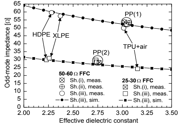
Fig. 6. Measured and simulated odd-mode impedance as a function of the effective dielectric constant for 25-30 \Omega FFCs and for 50-60 \Omega FFCs.
