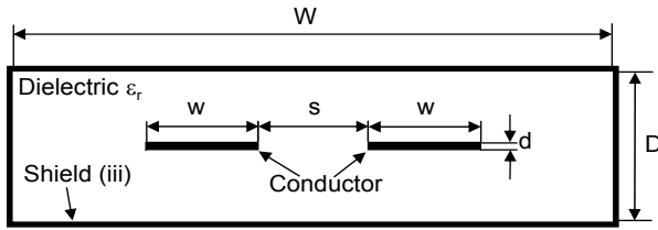
Fig. 3. Cross-sectional view of shielded FFC.
