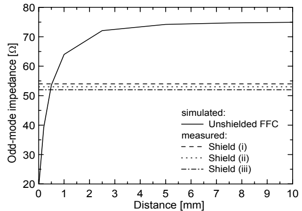
Fig. 1. Simulated odd-mode impedance as a function of the FFC-to-ground distance for an unshielded FFC. Measured Z_{\text{odd}} for 50-60 \Omega FFCs with shield (i)-(iii).
