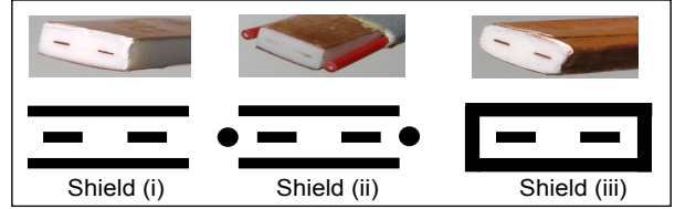
Fig. 5. FFC samples with three different shields were fabricated. The shield consists of copper foil that partially shields [(i) and (ii)] or fully surrounds the FFC (iii). The final coating process was not applied to these samples.
