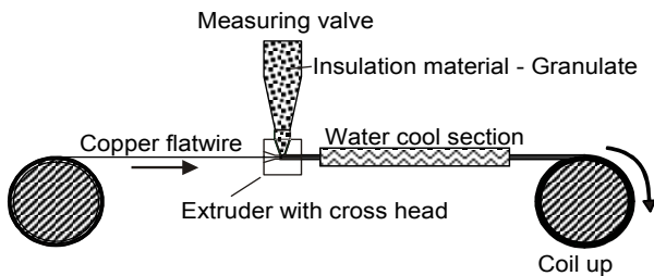
Fig. 4. Extrusion process: a flat wire is fed into an extruder where it is surrounded by melted granulates and finally cooled down.
