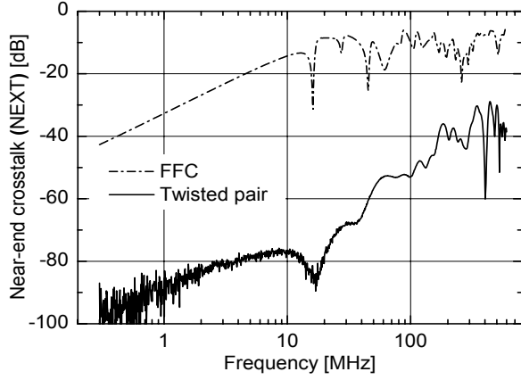
Fig. 2. Measured near-end crosstalk of two stacked FFCs compared to two twisted pair cables.
