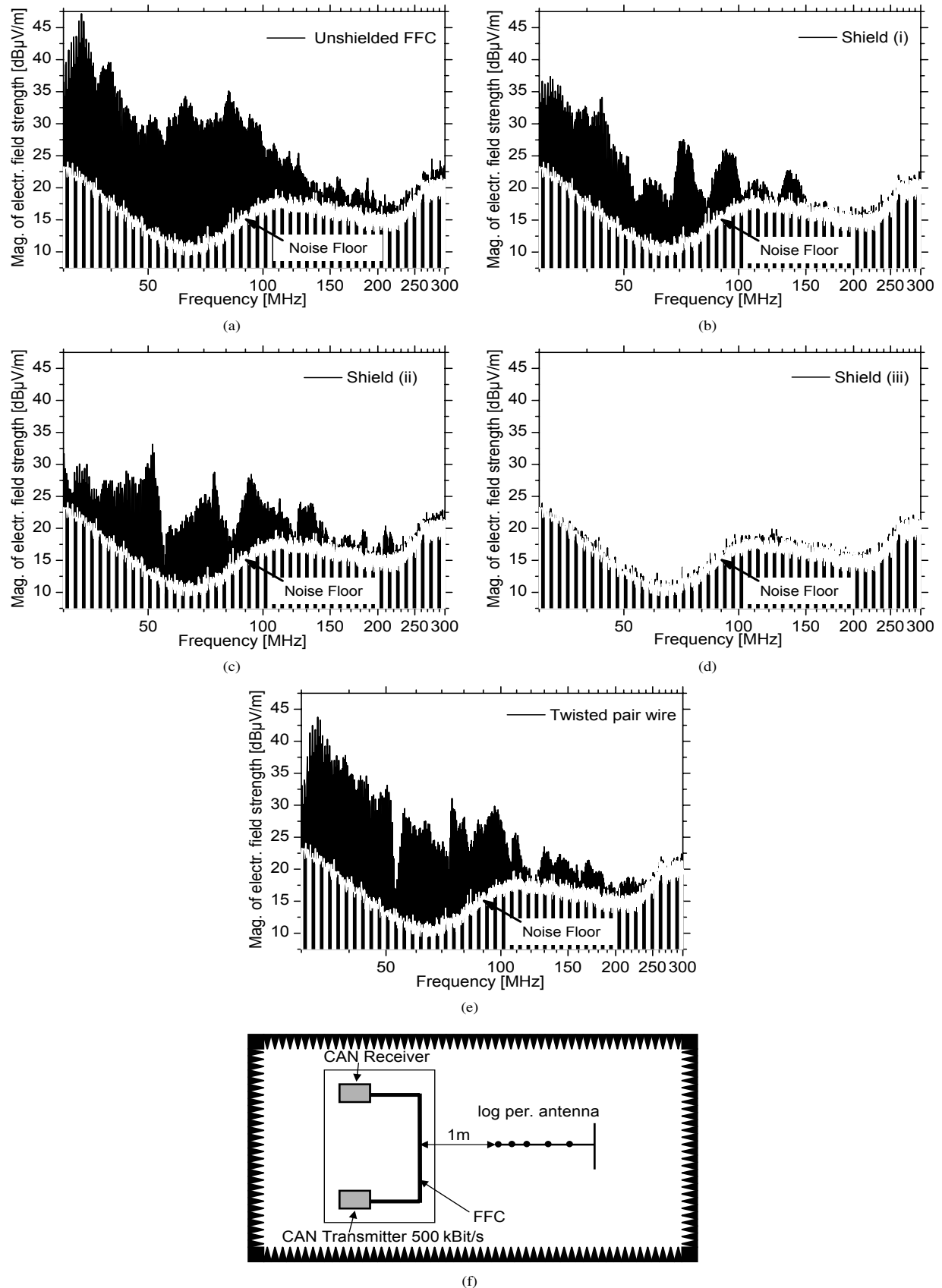
Fig. 7. Measured emission level as a function of frequency for two high speed CAN nodes connected with an unshielded FFC (a). (b) – (e) depict the emission results for shield (i) – shield (iii) and for a twisted pair wire, respectively. The measurement setup in the anechoic chamber is illustrated in (f) (top view).
