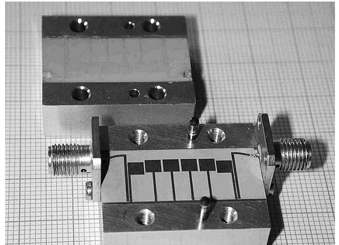
Fig. 10. Fabricated six-resonator filter.
