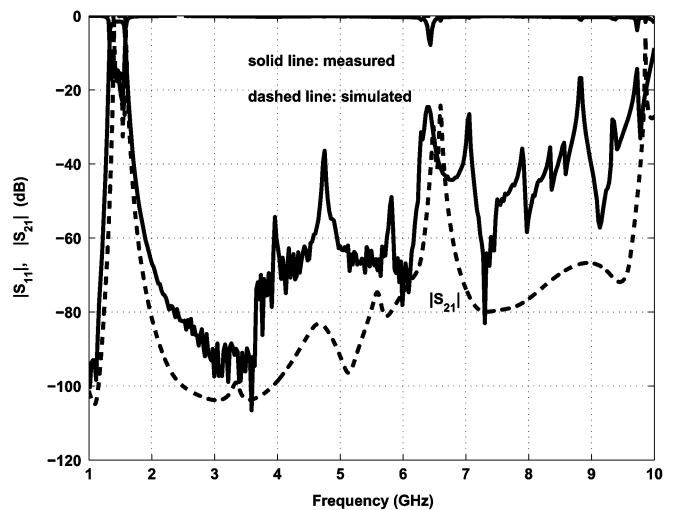
Fig. 11. Measured (solid lines) and simulated (dashed lines) frequency response of sixth-order harmonic-reject filter.
