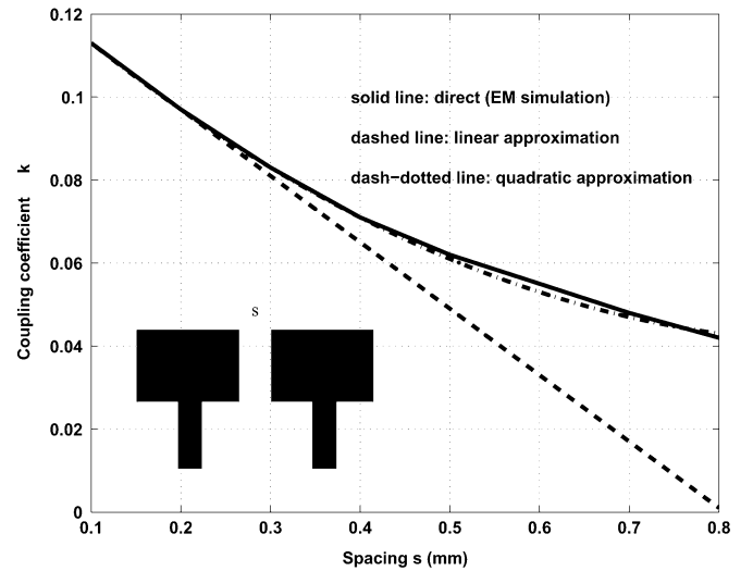
Fig. 3. Coupling coefficient versus separation distance between two resonators. Solid line: full-wave simulation. Dashed-dotted line: quadratic approximation. Dashed line: linear approximation.
