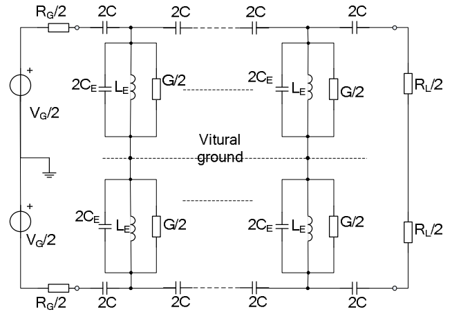
Fig. 3 Equivalent circuit of two lossy NRI TLs connected via the virtual ground
