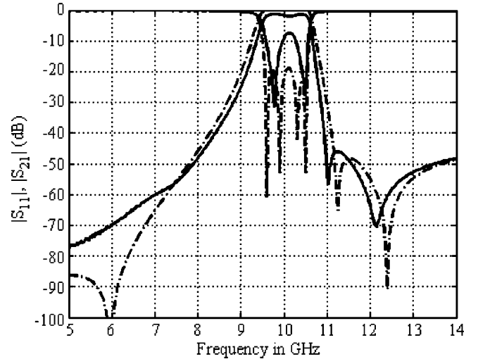
Fig. 17. Measured (solid lines) and simulated (dashed lines) results of fourth-order filter.
