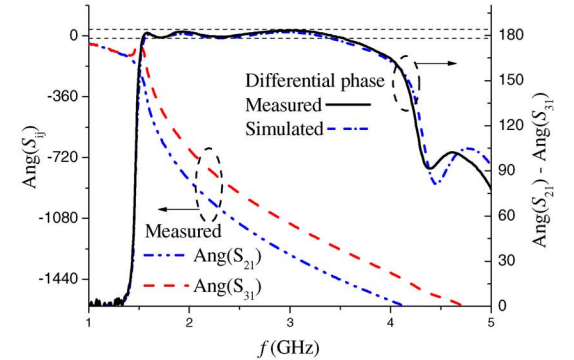
Fig. 4. Simulated and measured results of baluns A and B.
