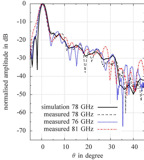
Fig. 8. Comparison of the measured (76, 78, 81 GHz) and simulated (78 GHz) radiation pattern in the cosecant 2 plane.
