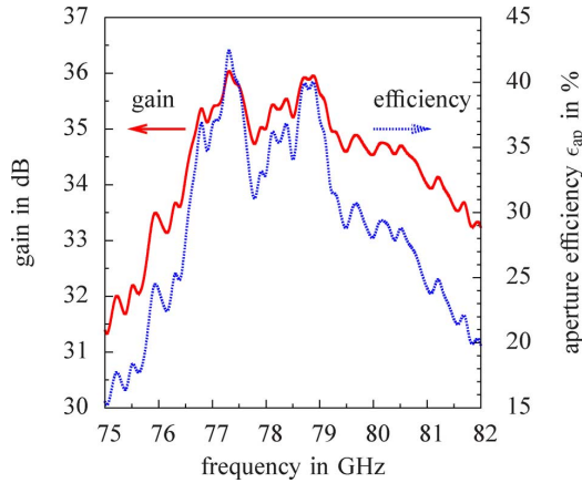
Fig. 5. Measured gain and resulted aperture efficiency.
