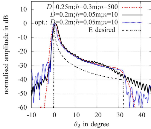
Fig. 4. Simulation results: cosecan squared pattern in elevation.
