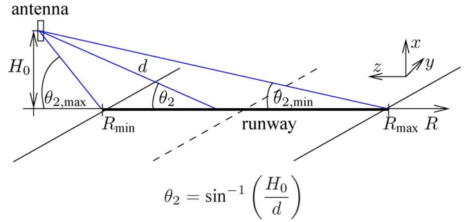
Fig. 1. Scenario for detecting objects on the runway.
