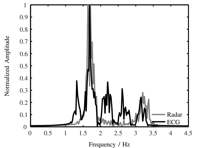
Fig. 7. Spectrum of the bandpass filtered heart beat signal in Fig. 6 after applying an additional second order notch filter in comparison with the spectrum recorded with an ECG.
