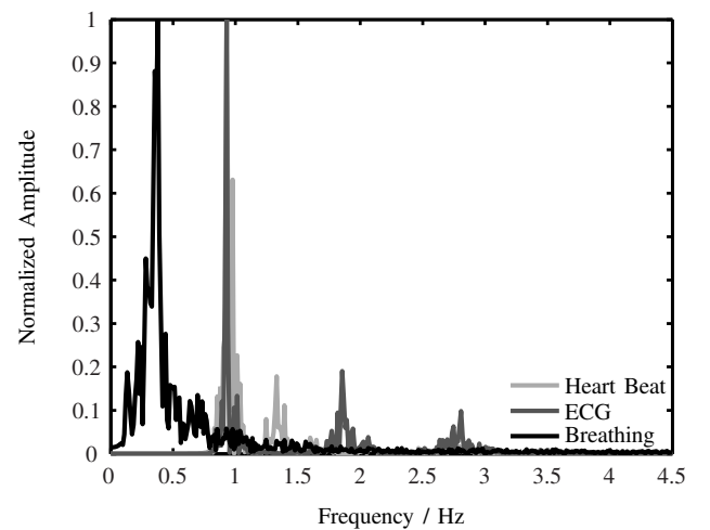
Fig. 4. Normalized spectrum of the recorded breathing and heart beat signal in Fig. 3 using a bandpass filter and comparison with the spectrum recorded with an ECG.
