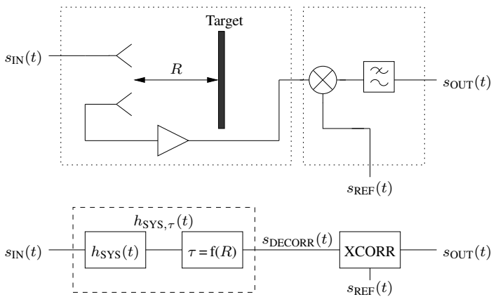
Fig. 9. Simplified block diagram of the UWB radar system (top) and mapping to its system theoretical description (bottom).
