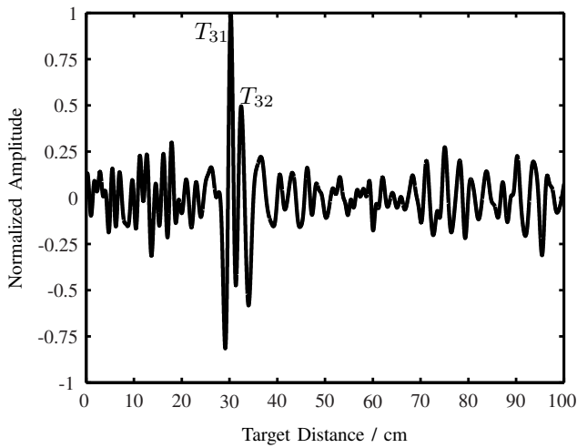
Fig. 12. Output signal after signal post-processing for a wooden board with a thickness of 17 mm as target.
