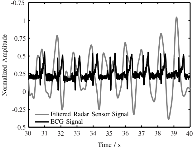
Fig. 5. Comparison of the filtered sensor output from Fig. 3 with the synchronously recorded ECG signal.
