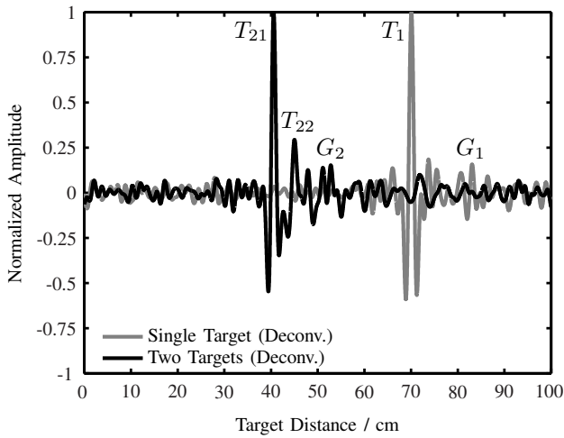
Fig. 11. Output signal of the raw data presented in Fig. 8 after application of the described deconvolution method.
