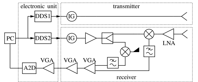
Fig. 2. Block diagram of the UWB radar system.
