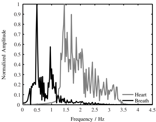
Fig. 6. Normalized spectrum for the measurement of a person after some sporting activities. A bandpass filter is applied to separate the breathing and the heart beat (1.1 Hz-4 Hz).
