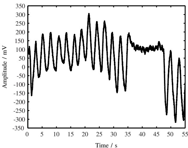
Fig. 3. Measured sensor output for a breathing person and a breath hold of about 12 s.
