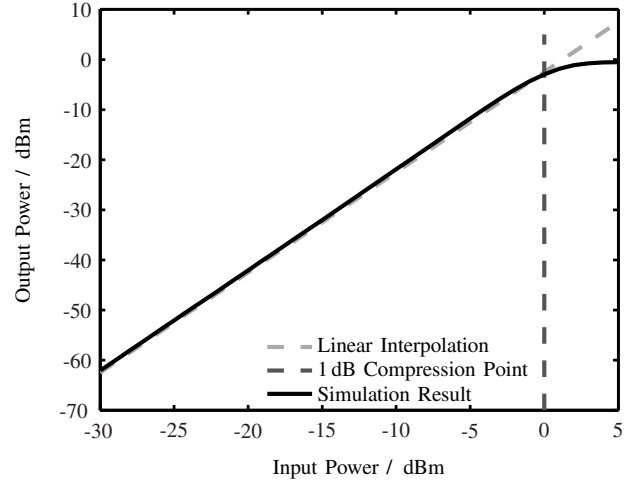
Fig. 3. Simulated output power of the squaring circuit at DC versus input power at 6.5 GHz.
