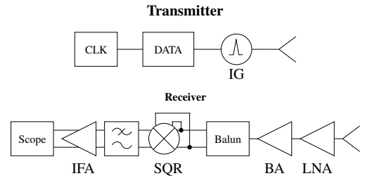
Fig. 1. Block diagram of the transmitter and the receiver.
