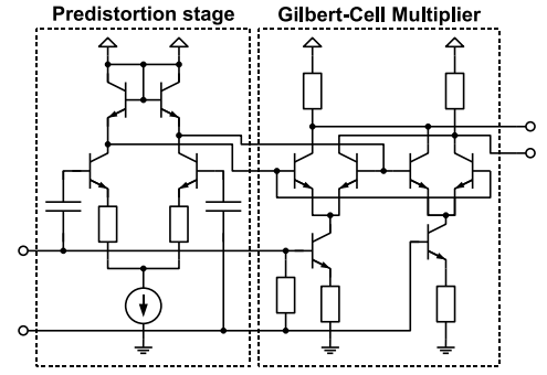
Fig. 2. Simplified schematic of the fully differential squaring circuit.
