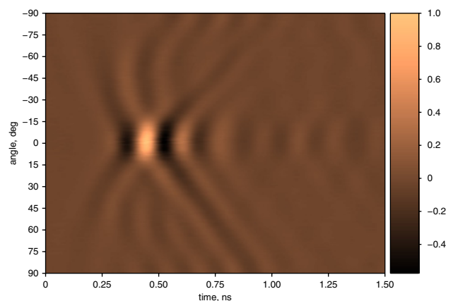
Fig. 3 Normalised received amplitude of antenna array with antenna spacing of 4 cm and no phase shift between trigger control signals
