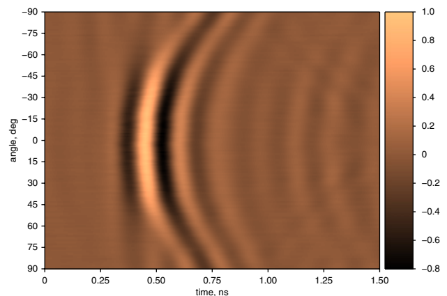
Fig. 2 Normalised received amplitude against H-plane rotation angle and time of single antenna element
