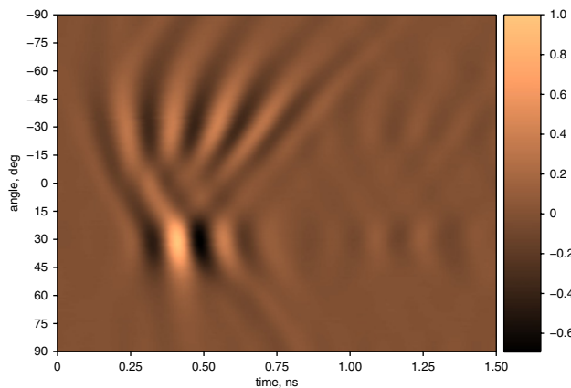
Fig. 4 Normalised received amplitude of antenna array with antenna spacing of 4 cm and phase shift for radiation angle of 30^\circ
