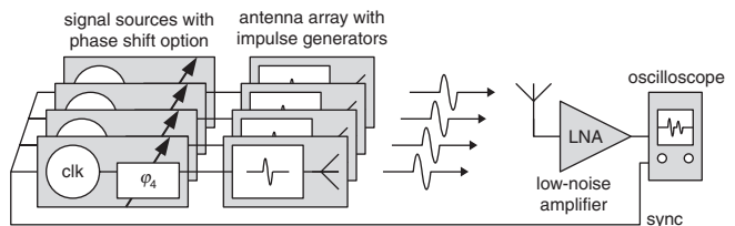
Fig. 1 Block diagram of proposed antenna array and measurement setup
