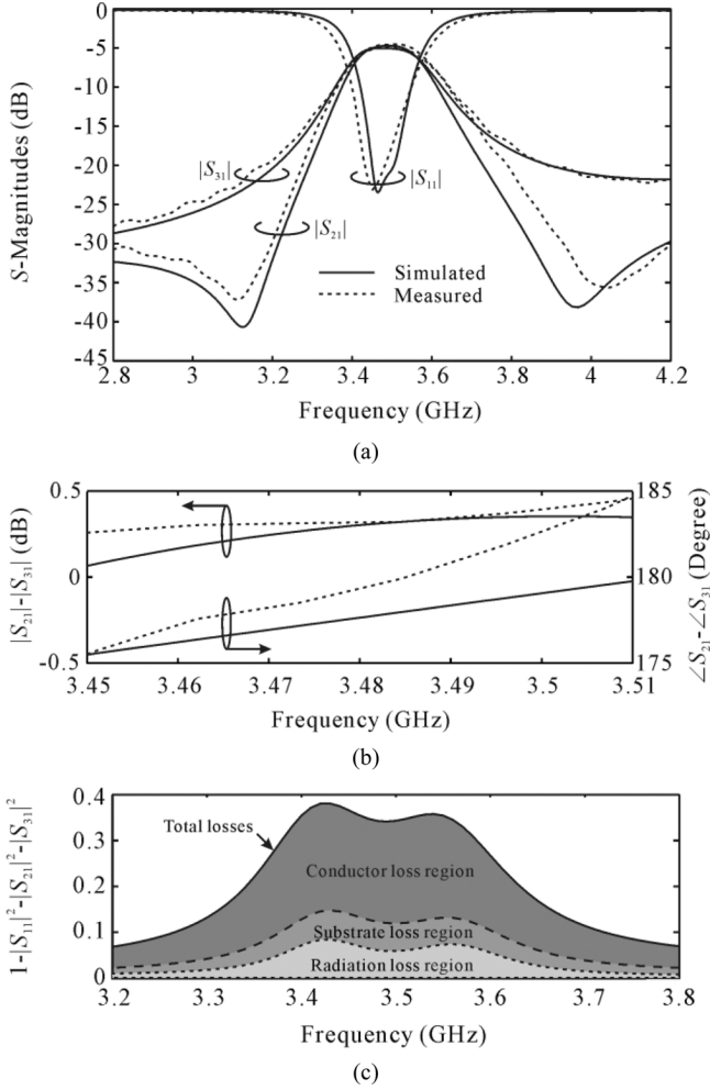
Fig. 5. Simulated and measured results of the designed balun-filter A. (a) S-Magnitudes. (b) Amplitude imbalance and phase balance. Dimensions: l_c = 7.0 , l_1 = 3.24 , l_2 = 2.16 , l_3 = 4.15 , l_4 = l_5 = 2.10 , l_6 = 2.12 , l_7 = 1.13 , w_1 = 0.26 , w_2 = 1.29 , w_3 = 0.10 , l_{s1} = 0.93 , l_{s2} = 1.40 . All are in mm. Material: \epsilon_r = 10.8 and thickness h = 0.635 mm, \tan \delta = 0.0023 , \sigma_{\text{Copper}} = 5.8 \times 10^7 S/m. (c) Simulated loss factors against frequency. EM simulator: Advanced Design System 2009.
