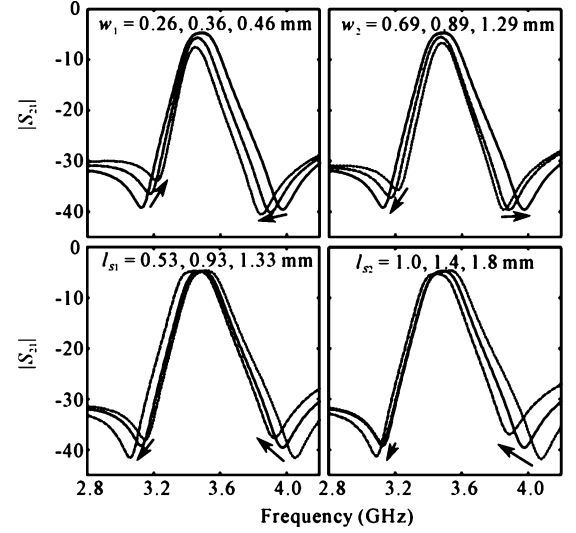
Fig. 3. Frequency responses with varied slot sizes ( w_1 and w_2 ) and stub lengths ( l_{s1} and l_{s2} ).
