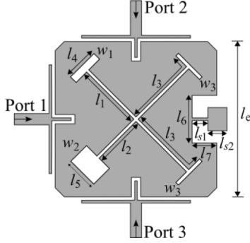
Fig. 1. Physical layout of the designed balun BPF.
