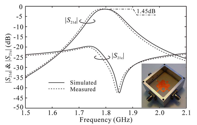
Fig. 6. Transmission responses of differential and common modes for balun-filter B with shielding box ( \sigma_{\text{Aluminum}} = 3.8 \times 10^7 S/m). Inset: Photograph of the fabricated shielded balun BPF. Dimensions: l_c = 14.0 , l_1 = 6.18 , l_2 = 2.98 , l_3 = 8.30 , l_4 = l_5 = 4.20 , l_6 = 4.24 , l_7 = 2.26 , w_1 = 0.72 , w_2 = 3.92 , w_3 = 0.20 , l_{s1} = 1.86 , l_{s2} = 2.85 . All are in mm. Material: \epsilon_r = 10.8 and thickness h = 1.27 mm, \tan \delta = 0.0023 .
