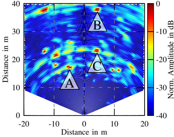
Fig. 7. Intensity plot of the measured scene obtained using linear prediction without target selection and with three targets marked according to Figure 6.
