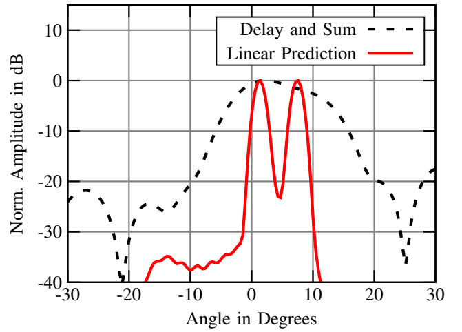
Fig. 3. Amplitude plot of a measured signal from two closely spaced corner reflectors using beamforming with delay and sum, and linear prediction.
