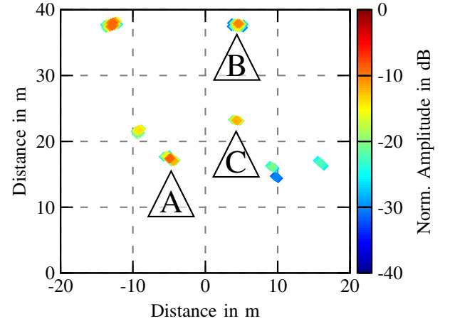
Fig. 8. Intensity plot of the measured scene obtained using linear prediction with target selection and with three targets marked according to Figure 6.
