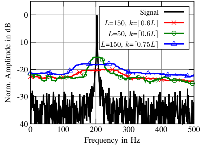
Fig. 5. Amplitude plot for a simulated signal with noise and the computed thresholds for different sets of CFAR parameters ( w=3.5 for all thresholds).
