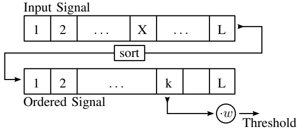
Fig. 4. Block diagram of the used OS-CFAR algorithm. X is the cell under test and k is the index of the selected noise sample in the ordered signal.
