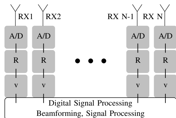
Fig. 1. Block diagram of the receive side of a digital beamforming radar sensor using N parallel receive channels.
