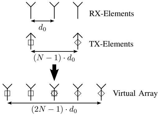
Fig. 2. Illustration of the DBF principle with synthetic aperture using three receive and two transmit elements [1].
