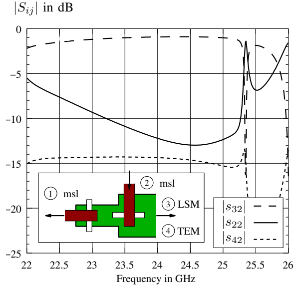
Fig. 3. Simulated S-parameters (insertion loss, return loss, excitation of the parallel plate mode (TEM)) of the transition microstrip line to the NRD-guide (LSM 01 mode).
