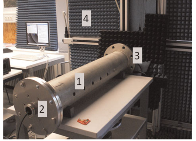
Fig. 6. Near-field measurement is set up to analyze a mode converter in a multimode pipe (1), with a diameter of 165 mm. The analyzed mode converter is mounted in the front-opening of the pipe (2). The field across the backside opening of the pipe (3) is analyzed with a near-field scanning probe of the near-field scanner in the background (4).
