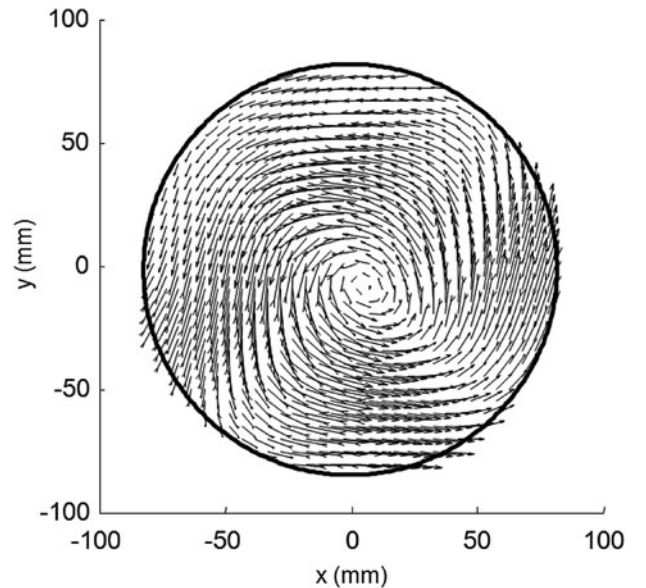
Fig. 7. Scanned near-field electric pattern of the overmoded waveguide at 5.8 GHz to measure the modes excited by the mode converter.
