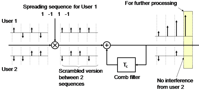
Figure 26. Illustration of multiuser interference suppression at the comb filter.
