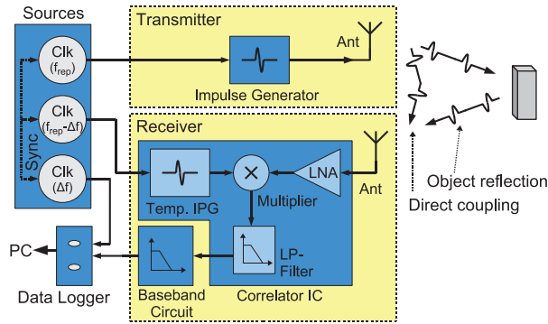
Figure 40. Block diagram of the single-ended bistatic radar system.
