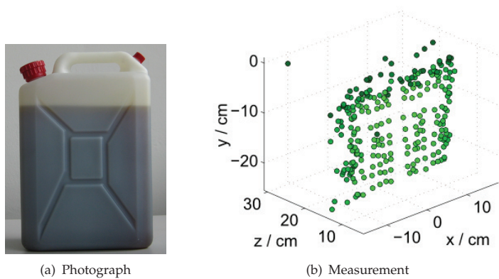
Figure 49. Photograph of the liquid container and measured cloud of estimated surface points.
