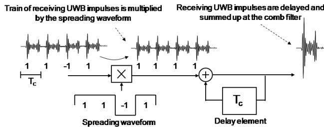
Figure 25. Comb filter principle in the receiver.
