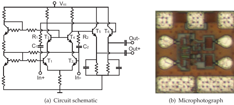
Figure 13. Complete circuit schematic and the chip microphotograph of the fully differential low-noise amplifier.
