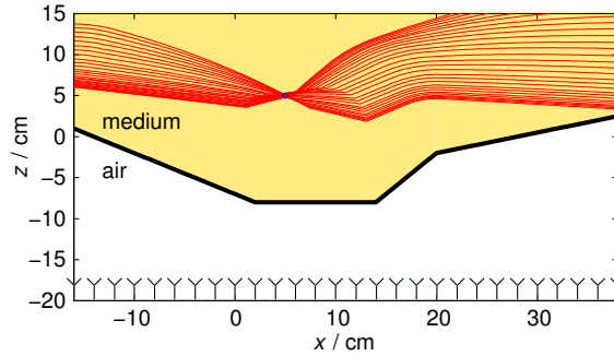
Figure 39. Calculated wavefronts in a medium with \epsilon_r = 10 based on EM field simulations. The receiving antennas are placed along the x -axis at z = -20 , the transmitter is positioned at (5 cm, 5 cm).
