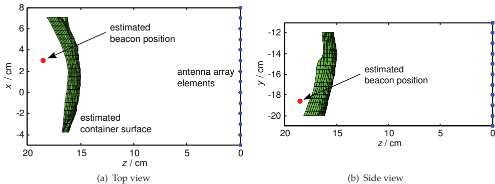
Figure 57. Measurement results in a top and side view corresponding to the photographs in Fig. 56 showing the estimated location of the beacon behind the container surface. The dots at z=0 represent the sensor positions.
