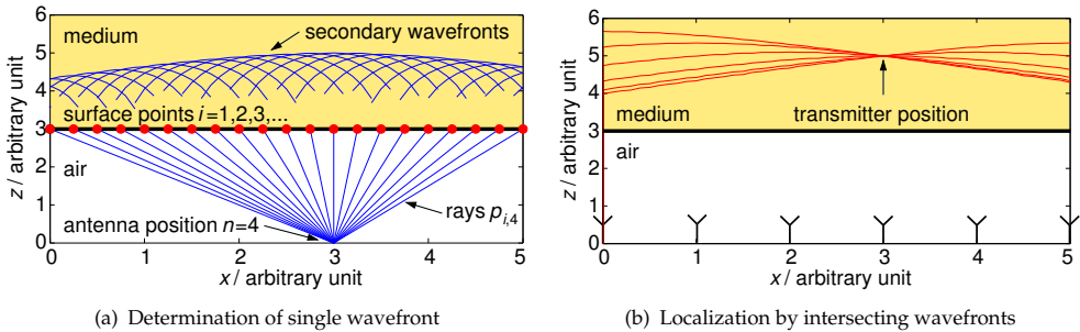
Figure 38. Determination of the 2D wavefront shape inside a medium with \epsilon_r = 30 for a signal transmitted in air at position (3,0) by evaluating the envelope of radial secondary wavefronts (a). Intersections of wavefronts corresponding to six different antenna positions indicate the transmitter location at (3,5) (b).
