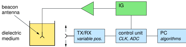
Figure 53. Measurement setup for surface estimation and subsurface transmitter localization. The radar sensor is moved in front of the liquid container to scan its surface. For localization, the upper part consisting of an impulse generator and an amplifier is switched on.
