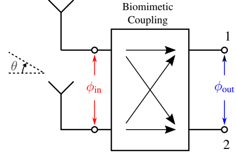
Fig. 1. Principle of the biomimetic antenna array (BMAA).
