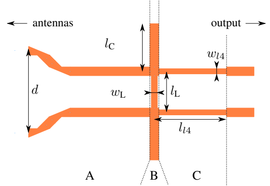
Fig. 7. Proposed coupling network scheme.
