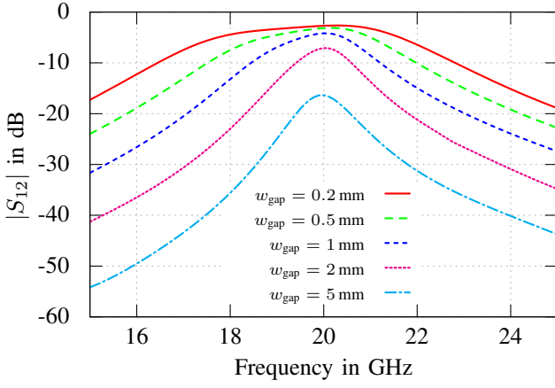
Fig. 5. Simulated |S_{12}| for different distances w_{\text{gap}} between the antenna elements. w_{\text{gap}} = 5 mm corresponds to an element distance of d = \lambda/2 .
