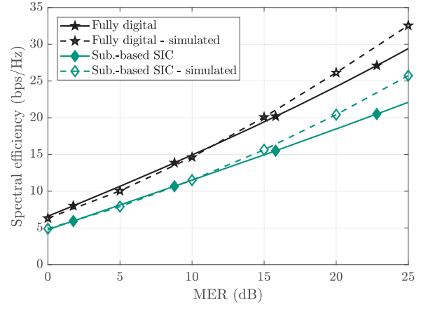
Fig. 3. Comparison of the spectral efficiency between the fitted curves based on the measurement data and the results gained from numerical analysis. For the numerical analysis the path-based MIMO channel model presented in [19] is employed, where the simulation parameters are adjusted to the findings obtained by channel measurements. The comparison is performed for the fully digital architecture and subarray-based hybrid beamforming architecture using the best performance algorithm presented in [8].
