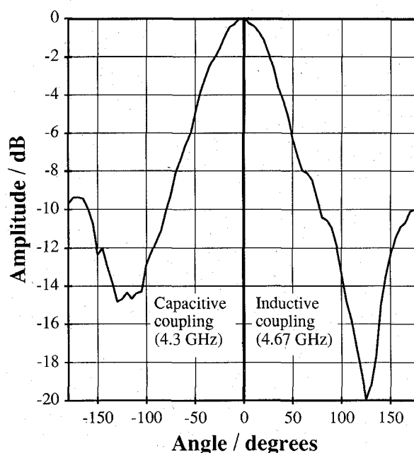
Fig. 5. H -plane radiation pattern for patch antenna with capacitive (left side) and inductive (right side) slot coupling.
