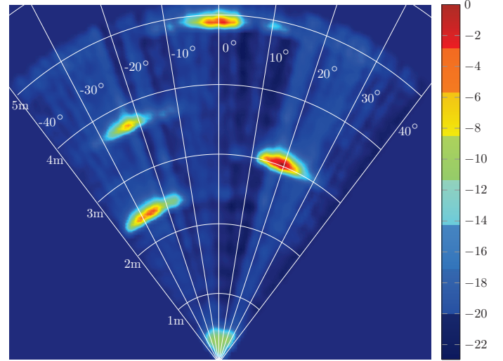
Fig. 9. 2-dimensional radar image of the measurement setup shown in Fig. 8 generated from 81 single envelope curves. The relative power is given in dB.
