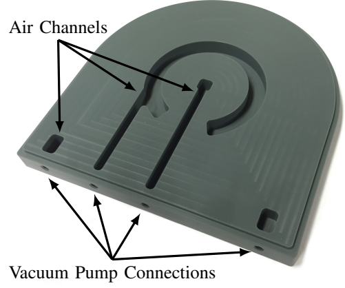
Fig. 3. Bottom part of the PVC chuck.
