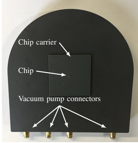
Fig. 4. PVC chuck with vacuum pump connections and chip.
