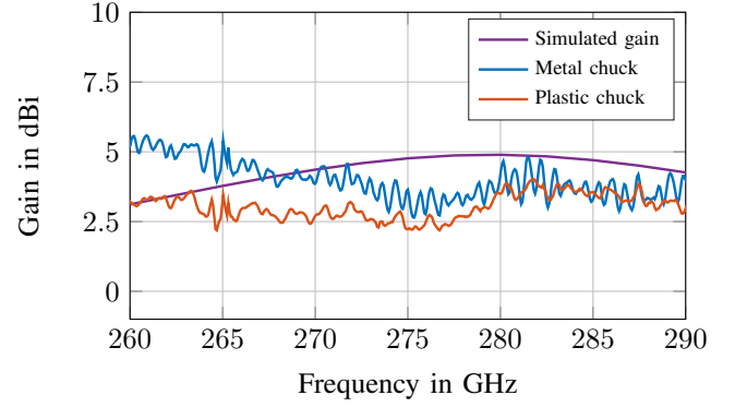
Fig. 10. Gain measurement of the integrated antenna with absorber at the Rx module.
