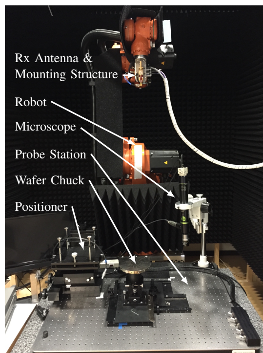
Fig. 1. Rx converter mount with reference antenna.
