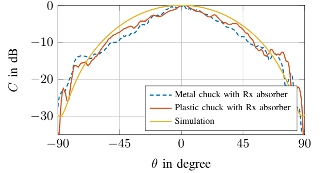
Fig. 7. Measurement of the integrated antenna in the H-plane with absorber at Rx module.
