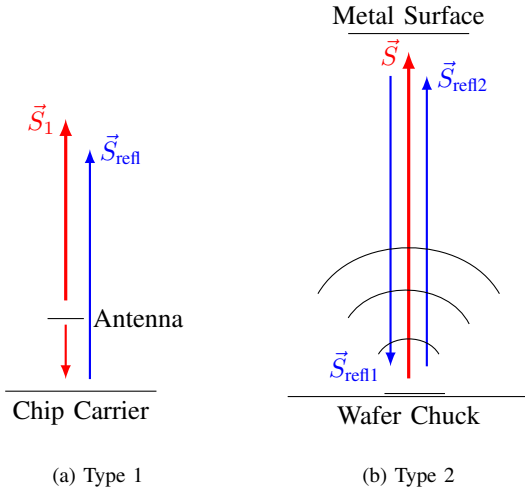
Fig. 2. Chuck reflections.
