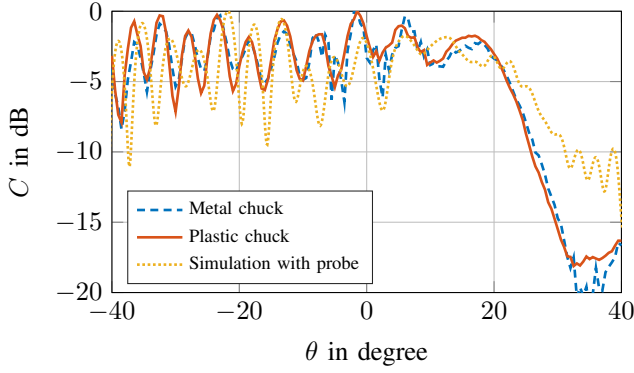
Fig. 8. Antenna pattern measurement in the E-plane with absorber at the Rx module.
