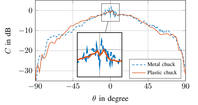
Fig. 6. Measurement of the integrated antenna in the H-plane.
