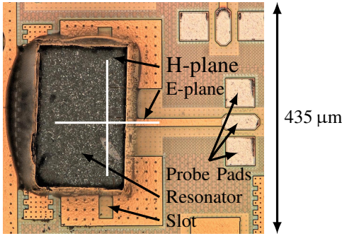
Fig. 5. Picture of the integrated antenna at 280 GHz.
