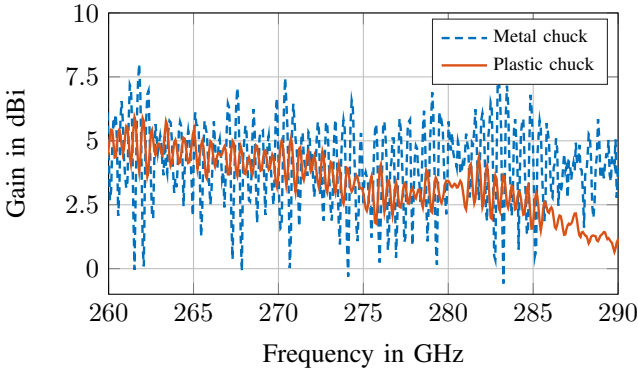
Fig. 9. Gain measurement of the integrated antenna without absorber at the Rx module.
