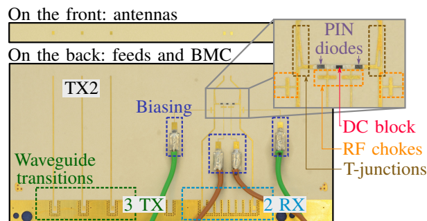
Fig. 5. Photography of the realized antenna board including the switchable two-element BMAA being the receive (RX) array. Only transmit (TX) antenna 2 is considered.
