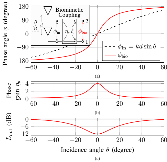
Fig. 1. Exemplary BMAA characteristics for an array with d = \lambda/2 , \eta = 4 , \xi = 0 (cf. [11]). (a) \phi_{\text{bio}} compared to the conventional phase progression kd \sin \theta , (b) the corresponding \eta_{\theta} , and (c) L_{\text{out}} (equivalent for both ports).
