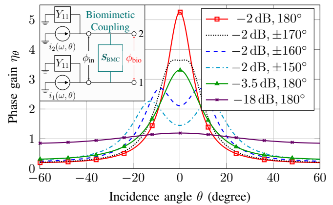
Fig. 2. \eta_{\theta} for a variation of S_{\text{BMC},21} for d = \lambda/2 and a fixed reflection coefficient of S_{\text{BMC},11} = (-50 \text{ dB}, 0^{\circ}) . Both transmission magnitude (solid lines) and phase (dashed/dotted lines) influence the phase gain of the BMAA. All curves are symmetrical to BS.
