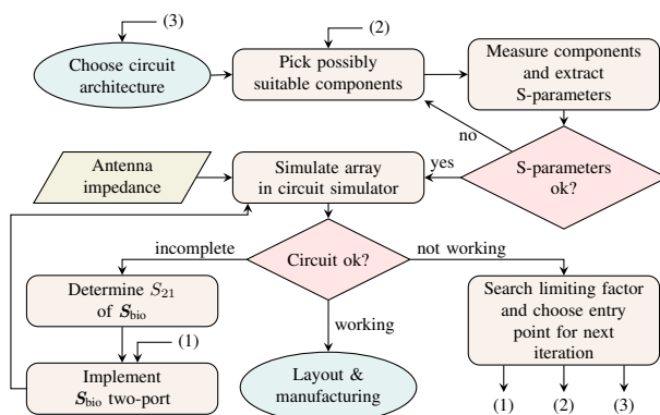
Fig. 4. Flowchart for the switchable BMAA design process.
