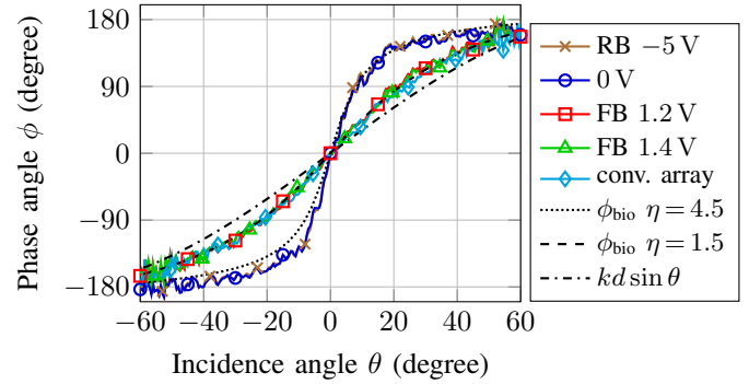
Fig. 7. Measured \phi_{bio} for four bias points. For 0 V and RB the array is switched to the BIO ON state. The array shows the same phase progression when forward-biased as when a conventional array without BMC is used.
