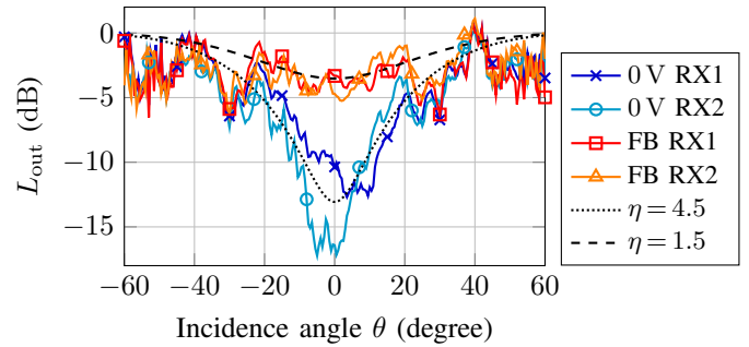
Fig. 8. Measured L_{out} of the two BMAA ports for 0 V and 1.2 V FB. When forward-biased the array does not show the typical angle-dependent power loss around BS. The theoretical curves for \eta = 1.5 and \eta = 4.5 (both \xi = 0 ) are identical for both ports.
